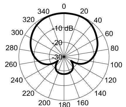
Polar diagram (both antennas)
